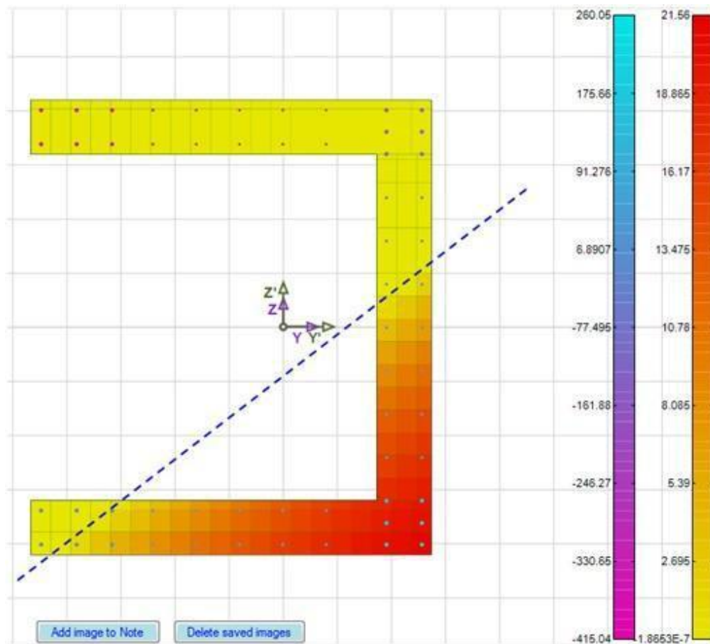
Real stresses (MPa) in concrete and reinforcement
